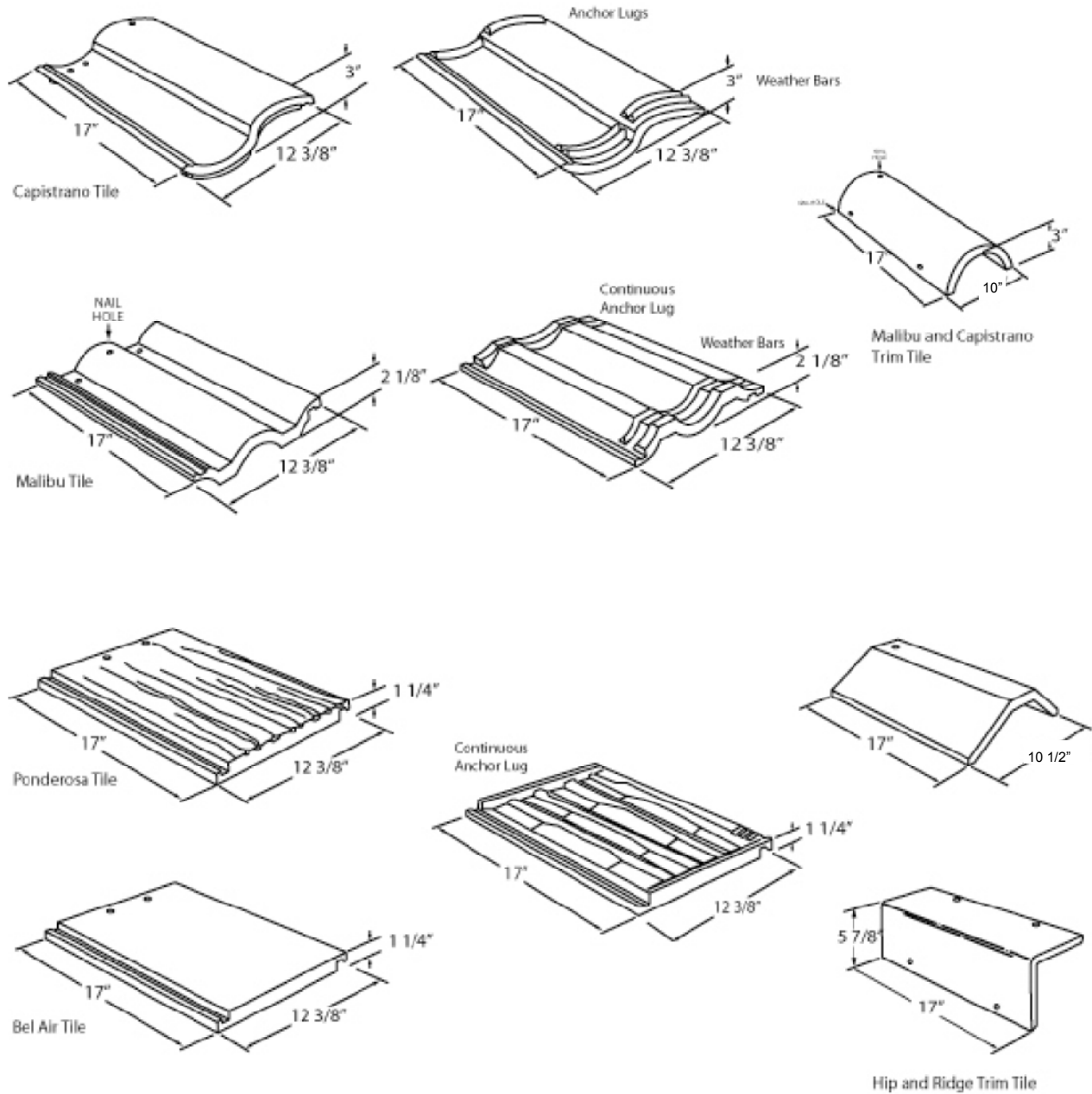
FIGURE 1—FIELD TILE AND TRIM UNITS
